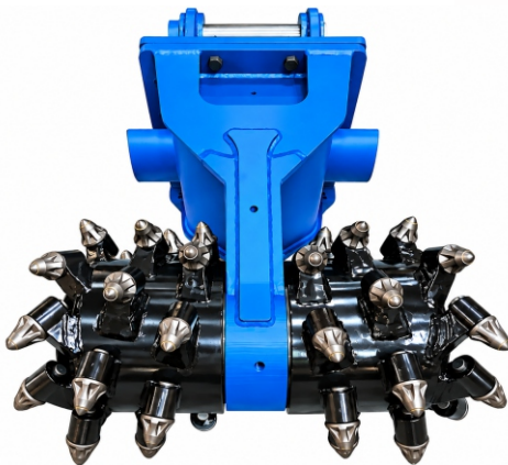
Drum Cutter
